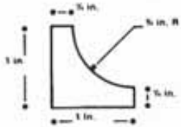
Trim "A"—Inside Corner Trim
