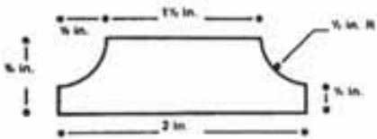
Trim "B"—Cap Trim
