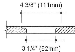
Sections showing water dam and drain details. (Lightweight option not shown)
