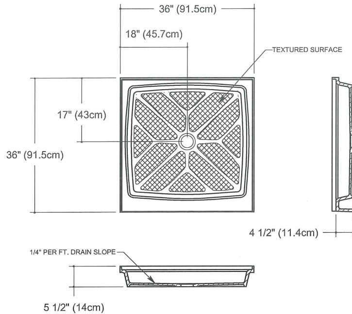
Sections showing water dam and drain details. (Lightweight option not shown)
