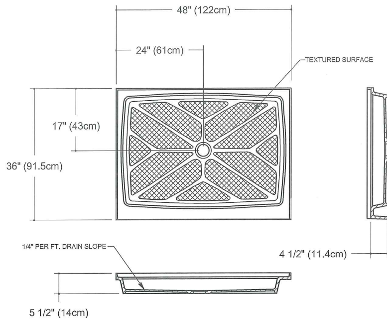
Sections showing water dam and drain details. (Lightweight option not shown)
