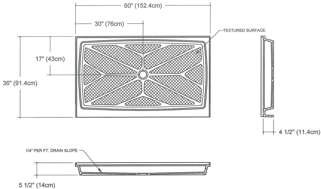
Sections showing water dam and drain details. (Lightweight option not shown)
